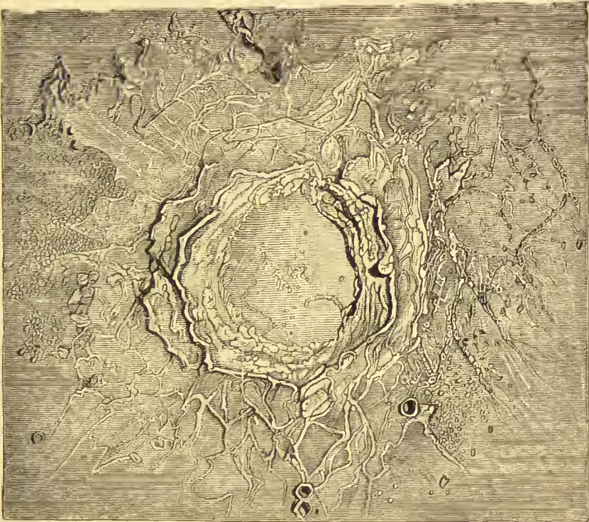
FIG. 40.—Another portion of the lunar surface, showing a so-called crater or vast lava pool and other evidences of ancient heat unmodified by water.
